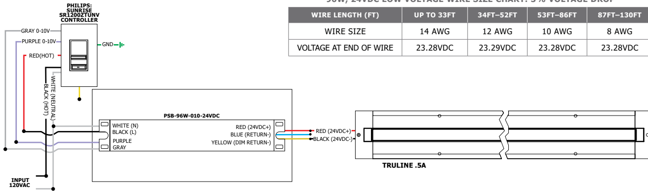
96W, 24VDC LOW VOLTAGE WIRE SIZE CHART: 3% VOLTAGE DROP
